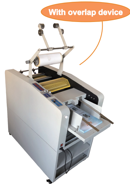
Suction Feeding AUTO-370S / AUTO-490S
