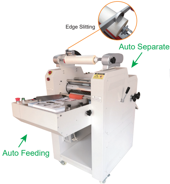
Friction Feeding AUTO-350
